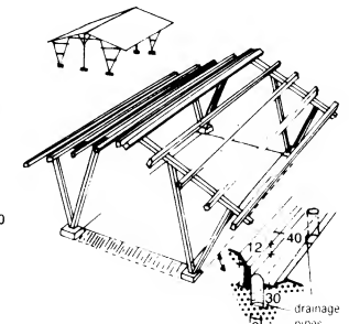
⑦ Field barn
